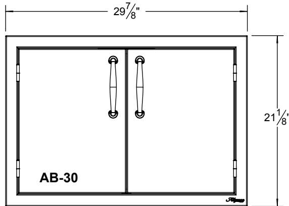
FRONT VIEW DOUBLE SIDED NARROW DOORS
